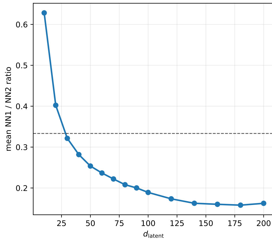
CelebA Encode-Decode Reconstruction Memorization
